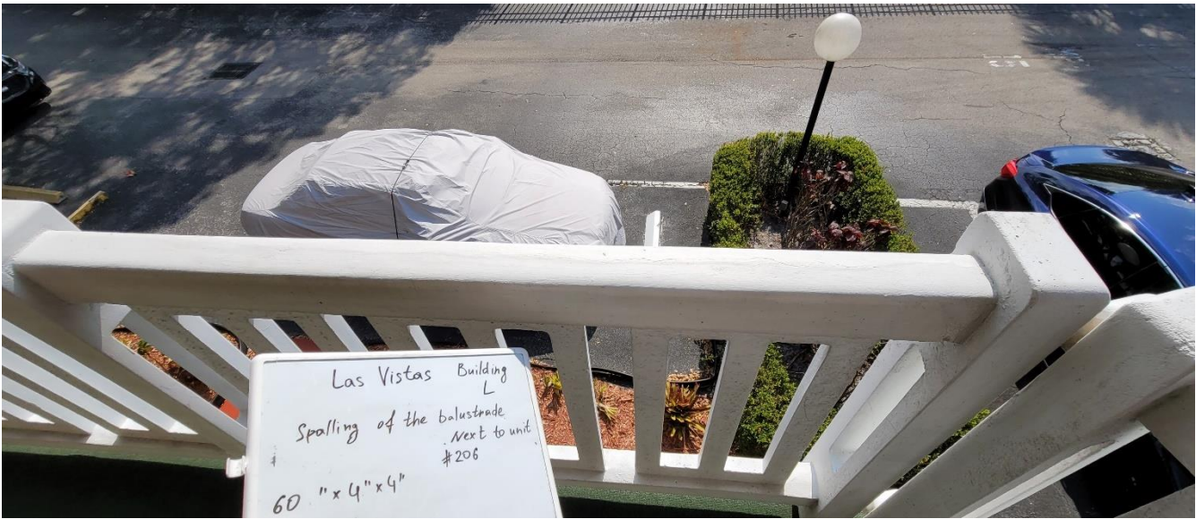
Spalling of the balustrade next to Unit 206
