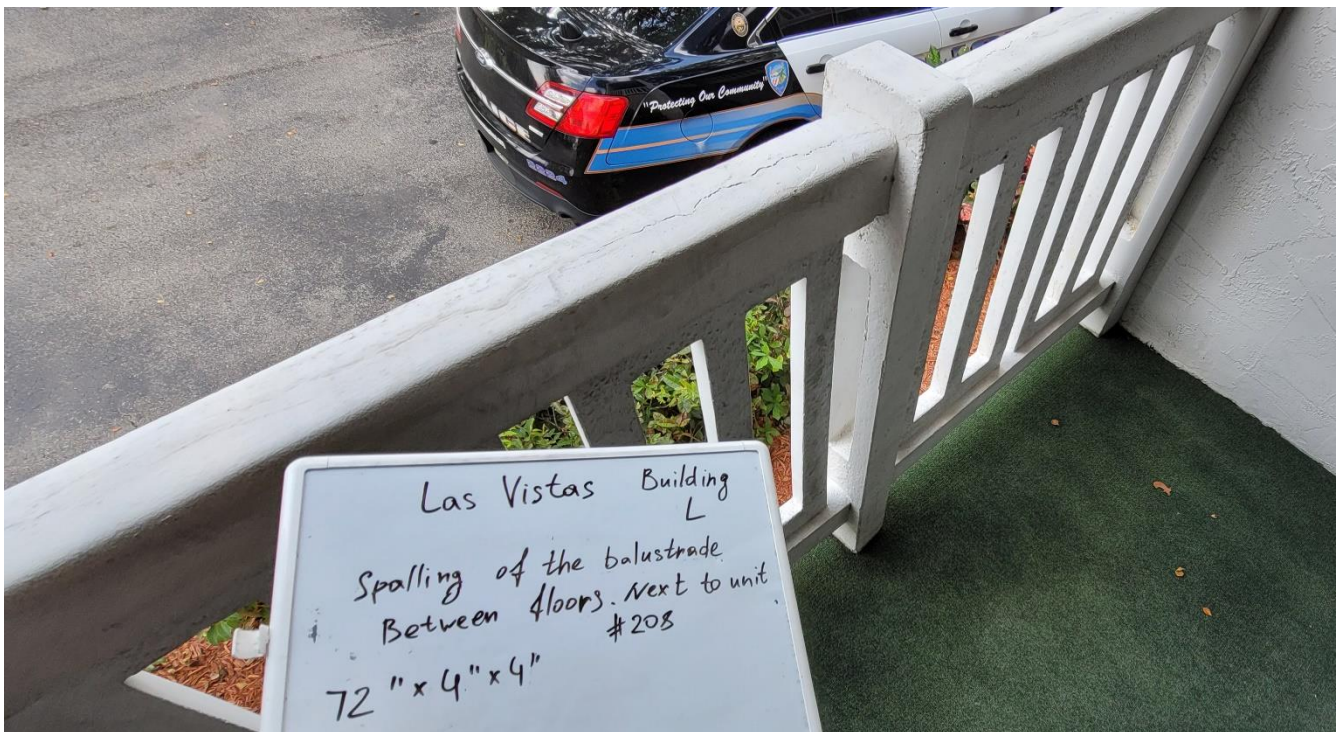
Spalling of the balustrade between floors next to Unit 208
