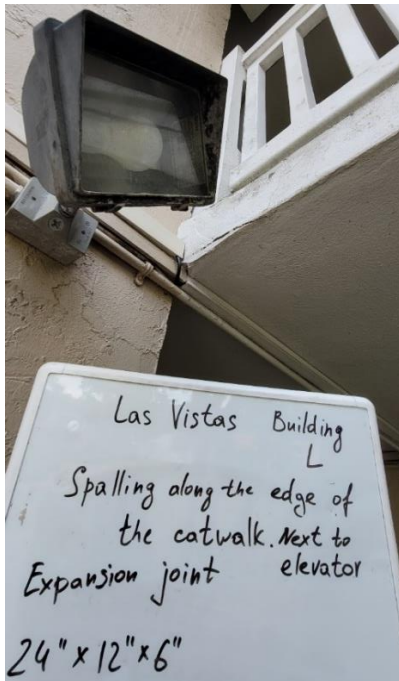
Spalling along the edge of the catwalk next to elevator
