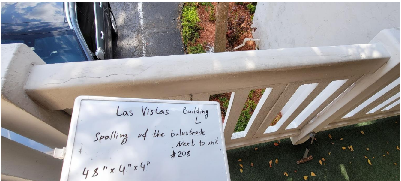
Spalling of the balustrade next to Unit 208
