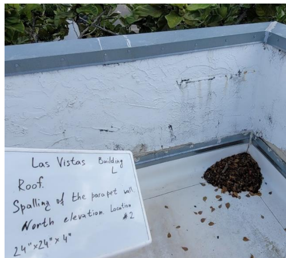
Spalling of the parapet North side
