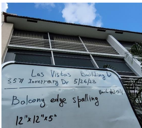
Balcony slab Unit 304
