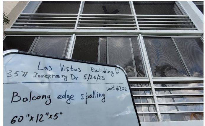
Balcony slab Unit 202
