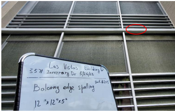
Balcony slab Unit 205
