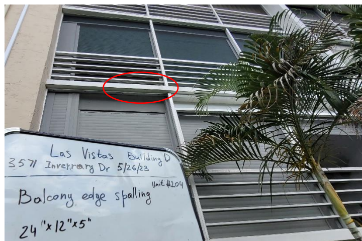
Balcony slab Unit 204
